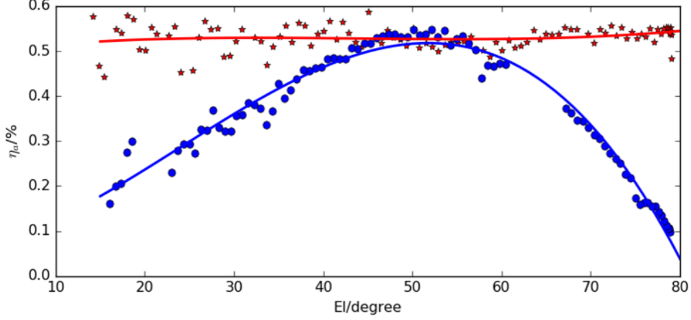
Figure 3: Elevation dependence of the aperture efficiency ( \eta_{\text{eff}} ) for Tianma telescope at Q-band. The red and blue colors represent \eta_{\text{eff}} with or without the active surface control, respectively.
