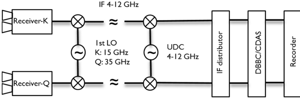
Figure 5: Flow diagram of signals from receiver to recorder for Tianma65.
