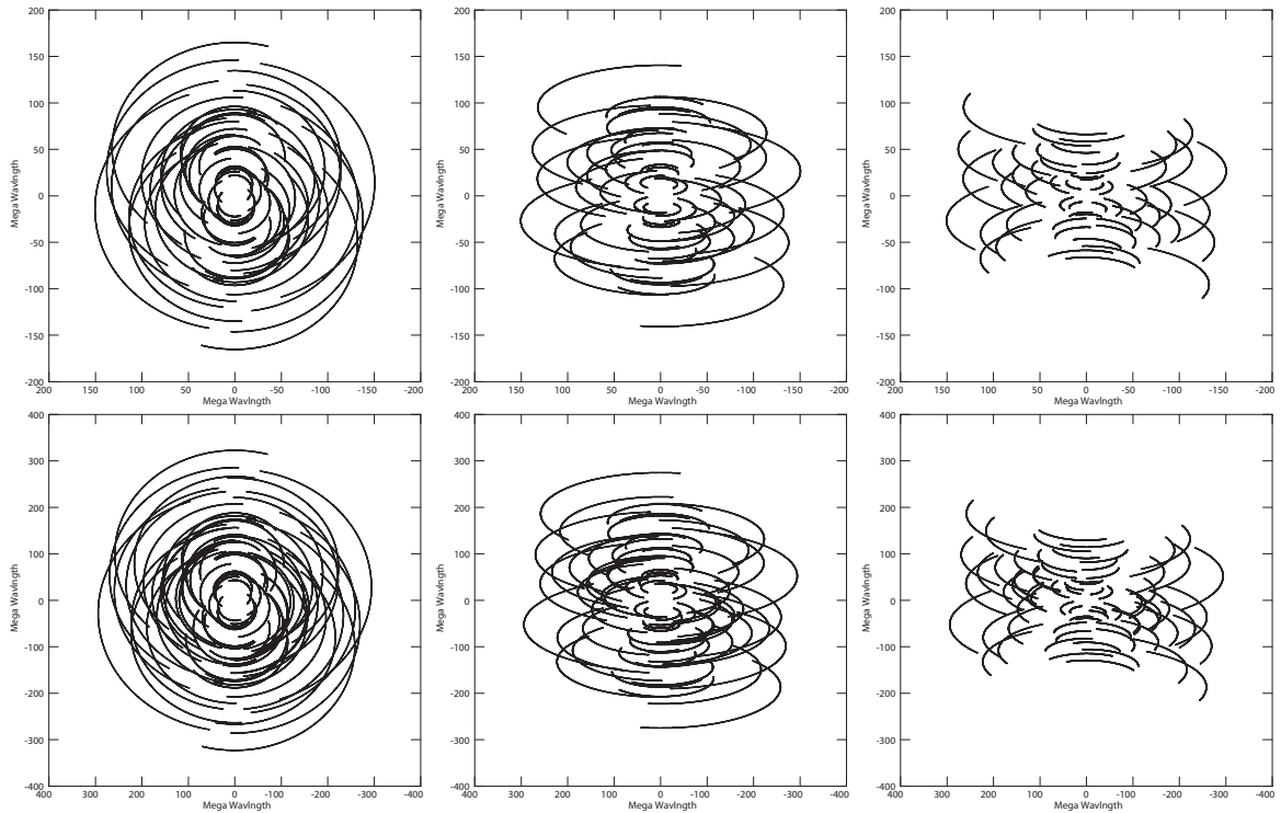
Figure 2: Examples of (u, v) coverage for an EAVN observation at 22 GHz (upper panels) and 43 GHz (lower panels) with the source’s declination of +60^\circ (left panels), +20^\circ (middle panels), and -20^\circ (right panels). Total observation duration of 10 hours is assumed for all cases.
