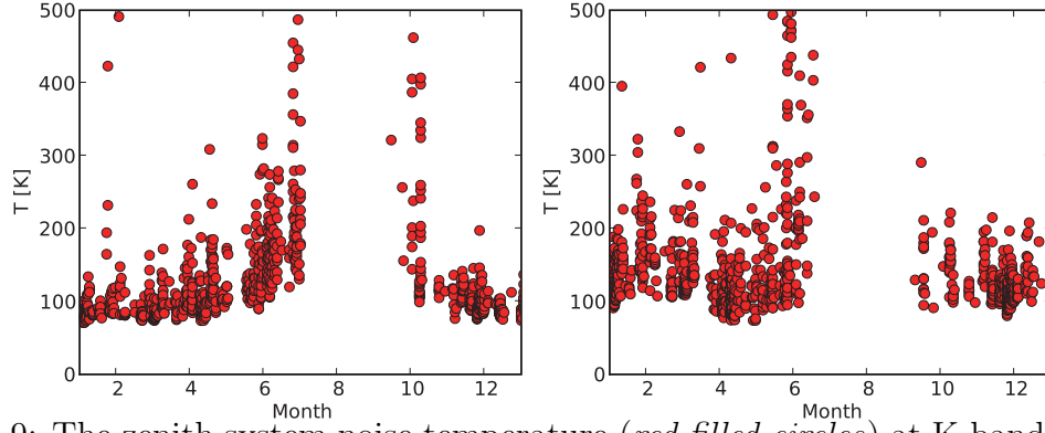
Figure 9: The zenith system noise temperature ( red filled circles ) at K-band (left) and Q-band (right) in KVN-Ulsan station.
