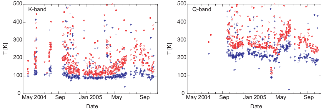
Figure 8: The receiver noise temperature ( blue crosses ) and the system noise temperature ( red open circles ) at the zenith at K-band (left) and Q-band (right) in VERA-Mizusawa station.
