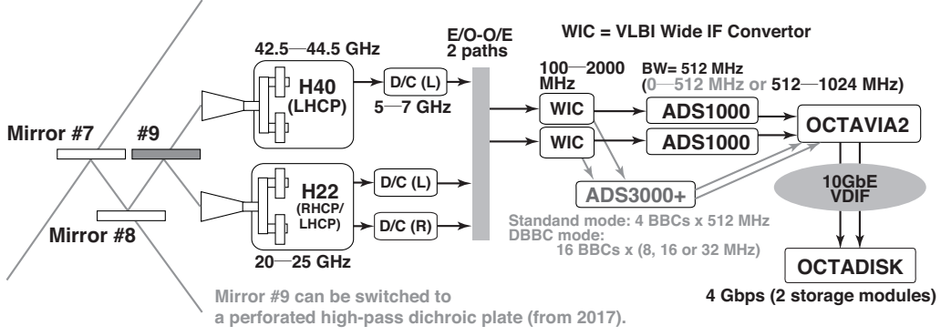
Figure 4: Flow diagram of signals from receiver to recorder for NRO45. Note that only the Q-band receiver is available for the EAVN 2018B open-use operation.
