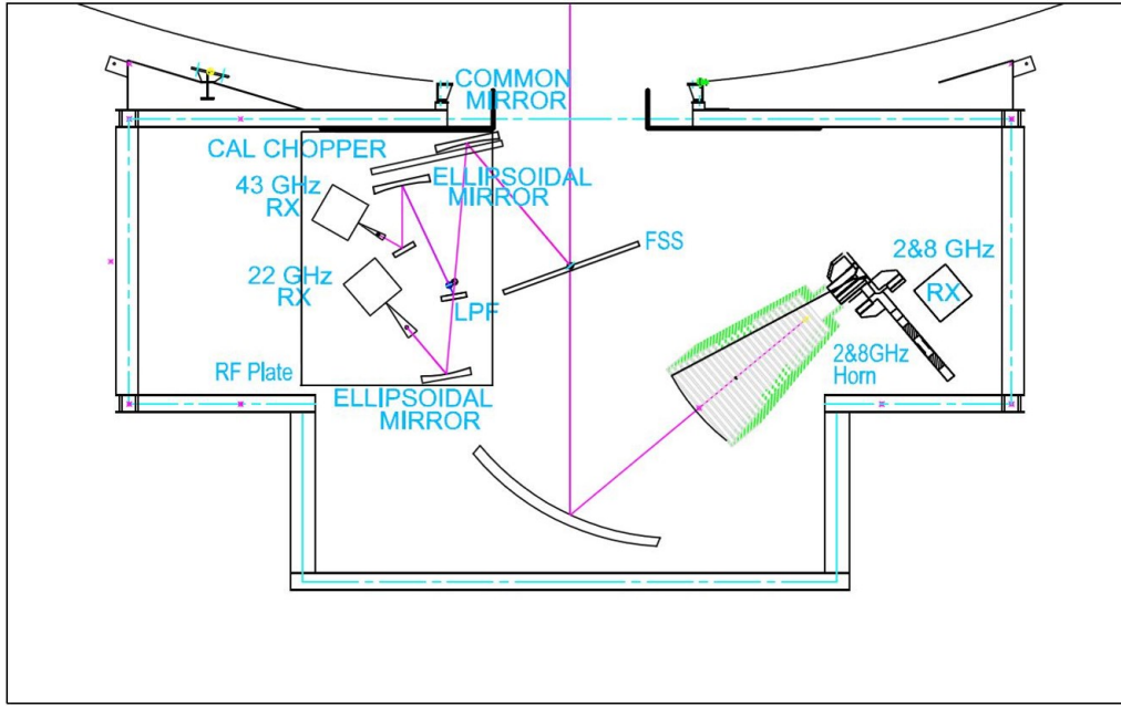
Figure 20: The KSJ quasi-optics and receiving system
